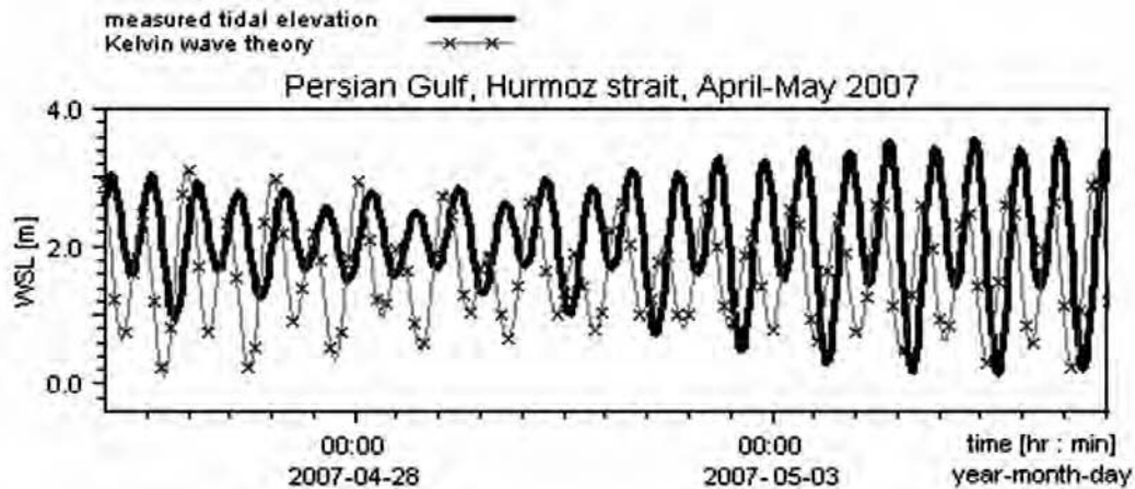
Fig. 7—Computed and measured tidal elevation at Didiamar Island.
