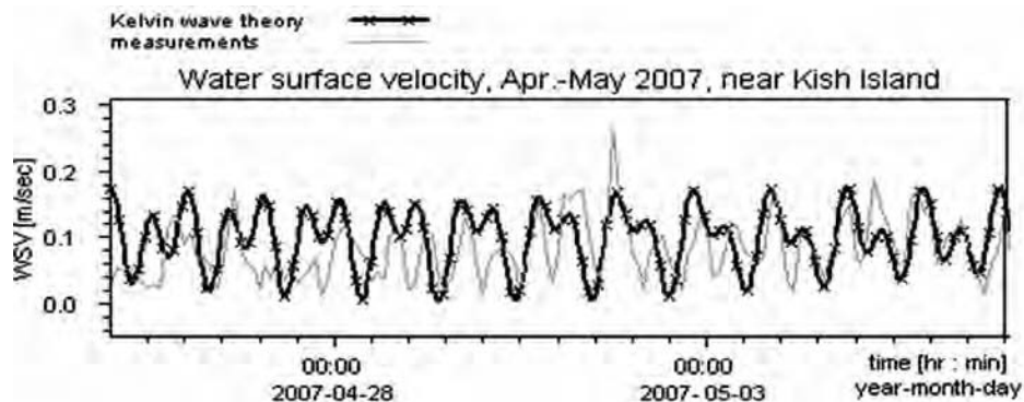
Fig. 9—Measured and computed surface velocity at Kish Island.
