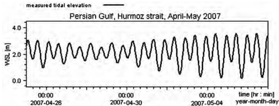
Fig. 3—Surface level fluctuations at Didamar Island, imposed at Hurmuz strait.
