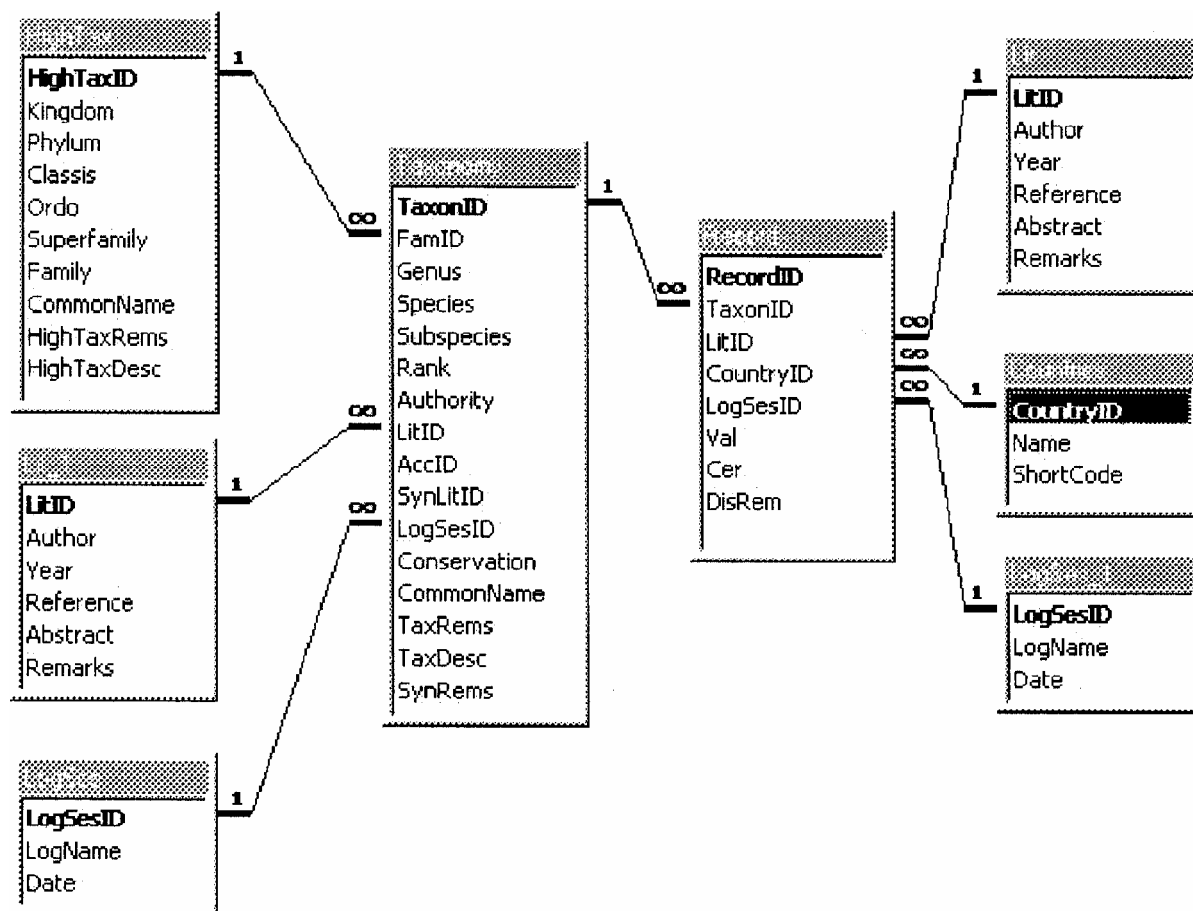
Fig. 1—Structure of the MASDEA database
