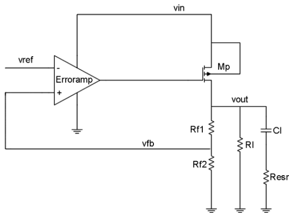
Fig. 1 – LDO voltage regulator 3
