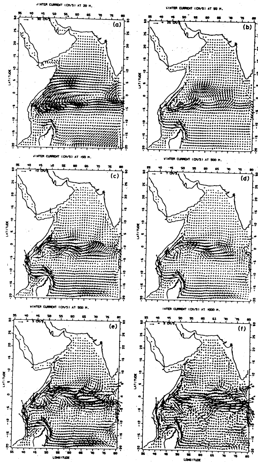
Fig. 5—Hydrodynamically adjusted currents (cm sec -1 ) during winter season using semi-diagnostic model at (a) 20 m depth (b) 50 depth (c) 150 m (d) 300 m (e) 500 m (f) 1000 m depths.
