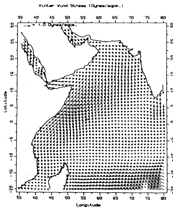
Fig. 1—Distribution of resultant wind stress (dynes \text{cm}^{-2} ) during winter season.
