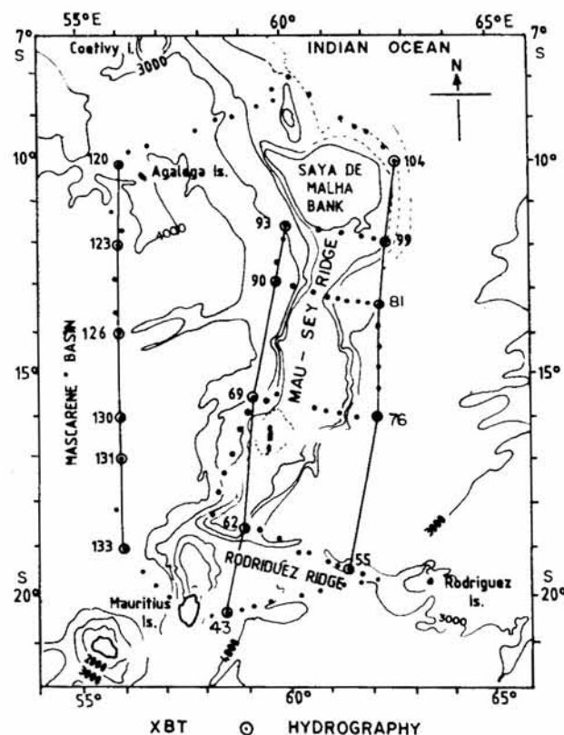
Fig. 1—Study area along with 3 meridional sections hydrography stations and XBT stations
