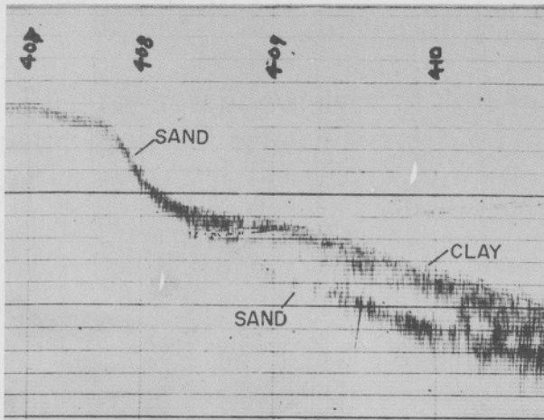
Fig. 3—Echogram showing the continuity of surface heavy mineral rich sand below layer
