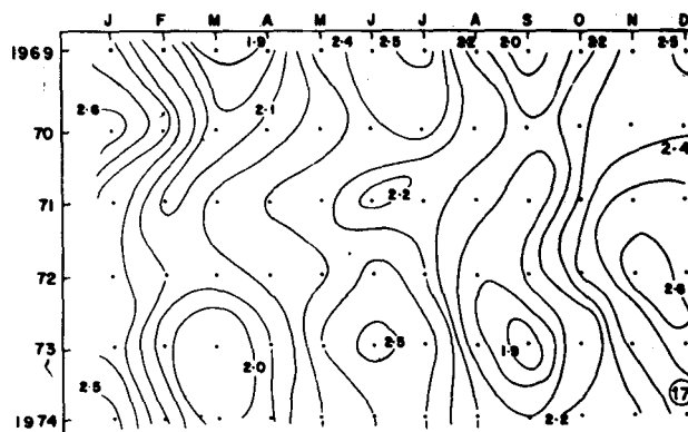
Fig. 17—Variations in tidal ranges as predicted for Mormugao Harbour (contour interval 0.1 m)
