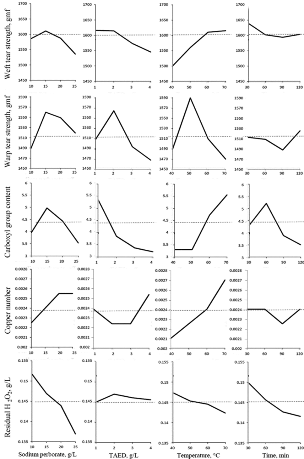
Fig. 2 — Effect of treatment condition on tear strength, carboxy group, copper number and residual peroxide of fabric (Main effect plots data mean values)
