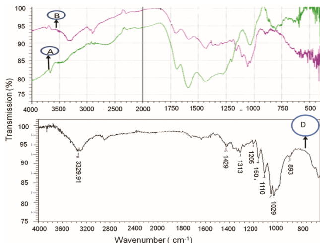
Fig. 6 — Char FTIR analysis of the control (A), BPS (B) and BPS+3% BA (D) treated cotton fabrics
