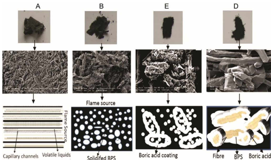
Fig. 5 — Char picture and morphologies of the control (A), BPS treated (B), BPS +1% BA (E) and BPS+3% BA (D) treated fabrics
