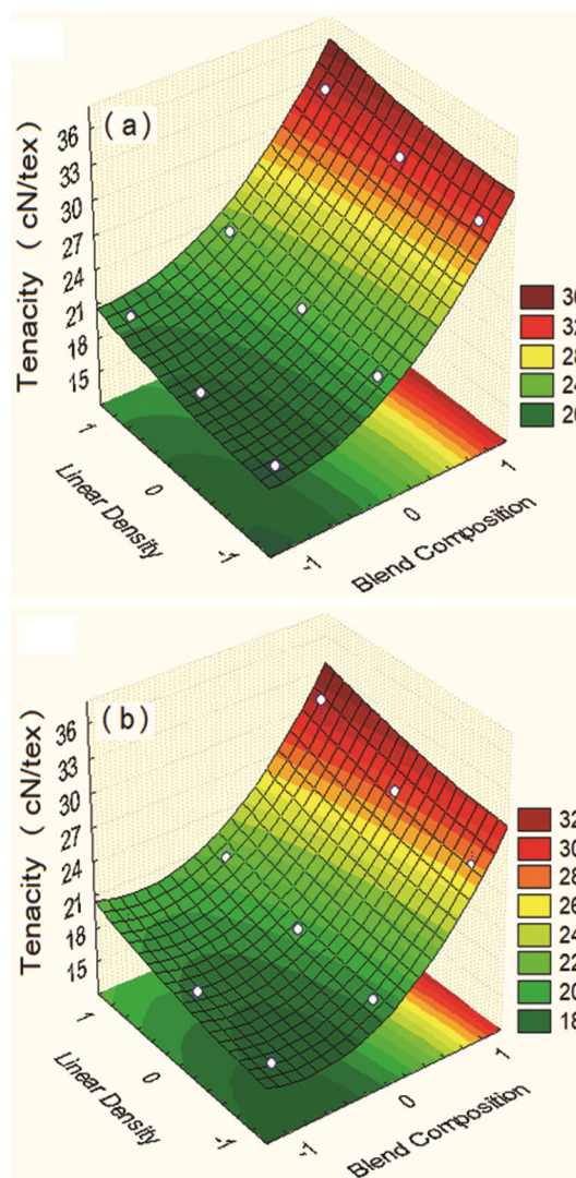
Fig. 6 — Influence of blend composition and linear density on tenacity of (a) Eli-Twist and (b) TFO yarns
