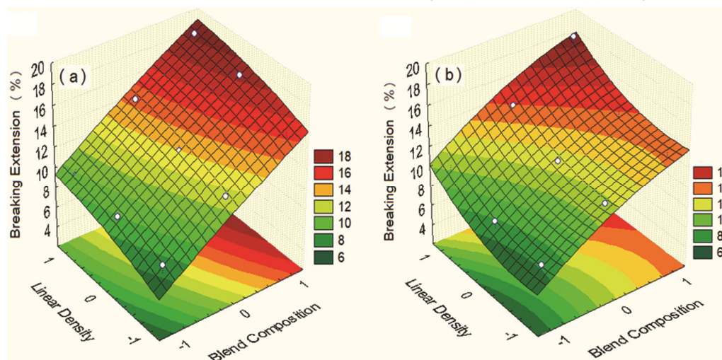
Fig. 7 — Influence of blend composition and linear density on breaking extension of (a) Eli-Twist and (b) TFO yarns
