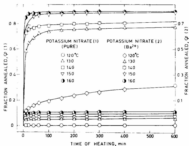
Fig. 1—Annealing of nitrite in gamma-irradiated pure and doped ( \text{Ba}^{2+} ) potassium nitrate.
