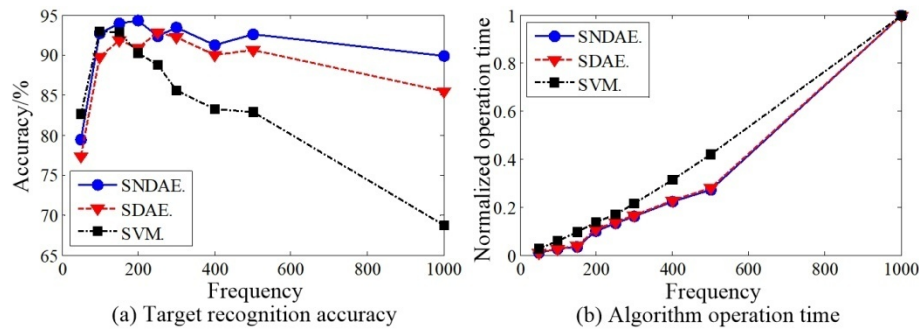
Fig. 10 — Curves of recognition accuracy and program run time changed with end frequency
