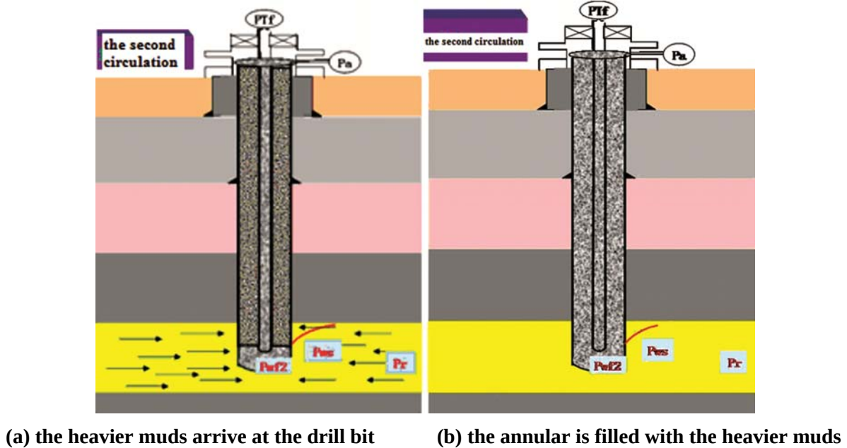
Fig. 2 — The second circulation of driller's method
