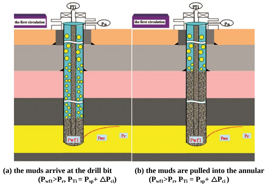
Fig. 1 — The first circulation of driller's method
