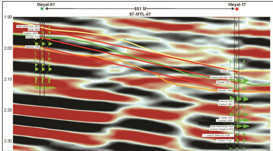
Fig. 5 — Synthetic of wells Meyal-01 and Meyal-17
