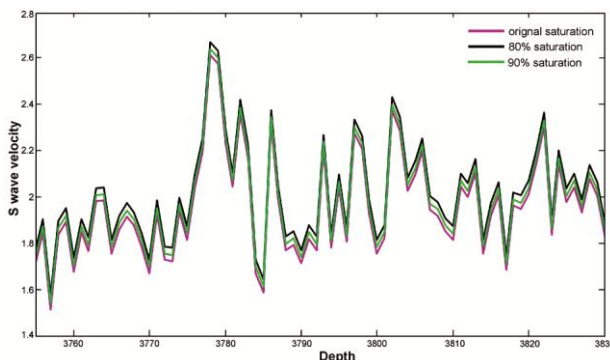
Fig. 11 — Variation of S-wave velocity at different levels of saturation
