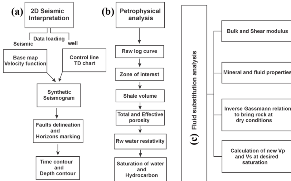
Fig. 4 — Work flow: (a) Seismic interpretation, (b) Petrophysical analysis, and (c) Fluid substitution
