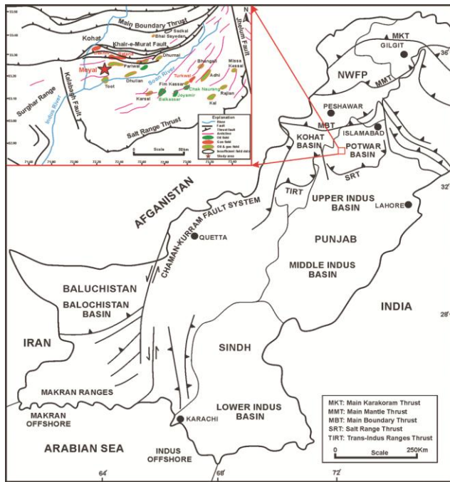
Fig. 1 — Generalized tectonic map of Pakistan showing Sedimentary Basins (Modified in GIS 10 after Farah et al. 23 ). The red rectangle show the tectonic framework of the Potwar Basin where red star indicates the location of the study area
