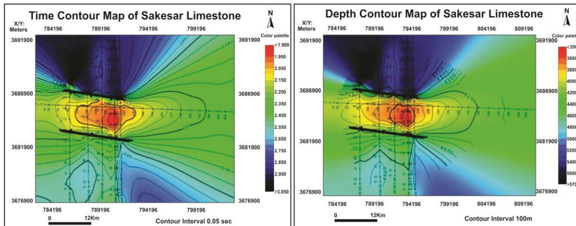
Fig. 7 — Time and depth contour map on top of marked horizon. Color bar represents variation of time and depths in seconds and meters respectively
