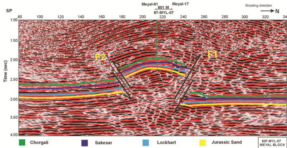
Fig. 6 — Interpreted seismic section with marked horizons and faults
