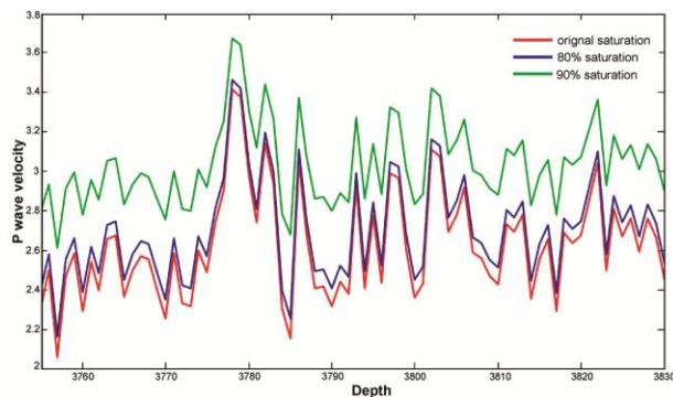
Fig. 10 — Variation of P-wave velocity at different levels of saturation
