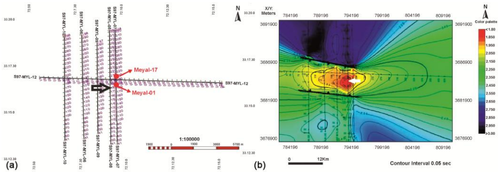
Fig. 8 — (a) New lead on base map along seismic line; and (b) Structural High on time contour map
