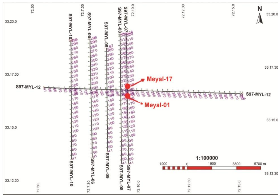
Fig. 3 — Base map of the study area showing location of seismic lines and well
