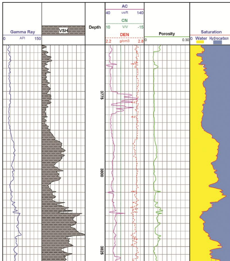
Fig. 9 — Petrophysical analysis of well Meyal 17
