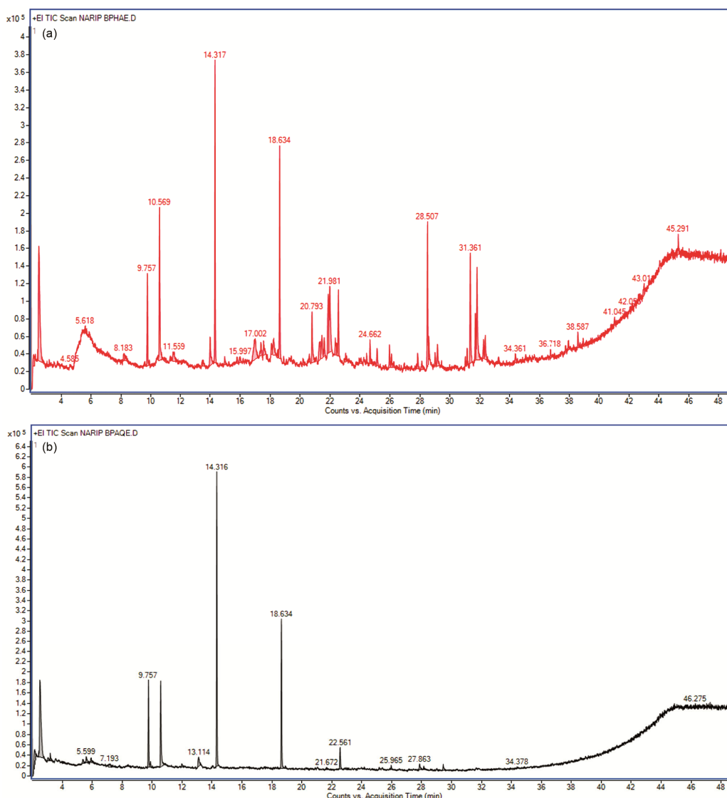
Fig. 6 — GC-MS Chromatogram of (a) HEBP, and (b) AEBP.
